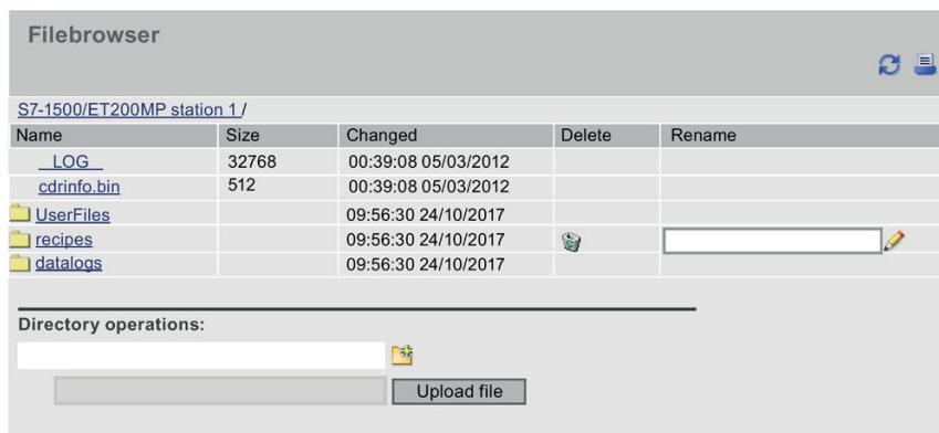
Figure 3-12 Standard "File browser" web page of the Web server
